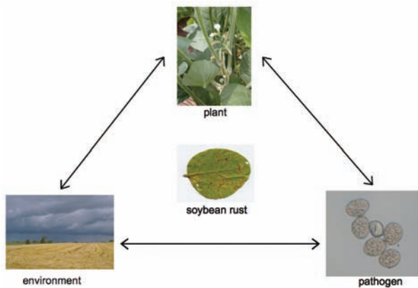
Figure 1. Disease triangle: A susceptible host plant, favorable environment, and the presence of the pathogen interact to produce disease. Soybean rust occurs during early reproductive growth stages, cloudy and rainy weather, and the presence of airborne spores.
